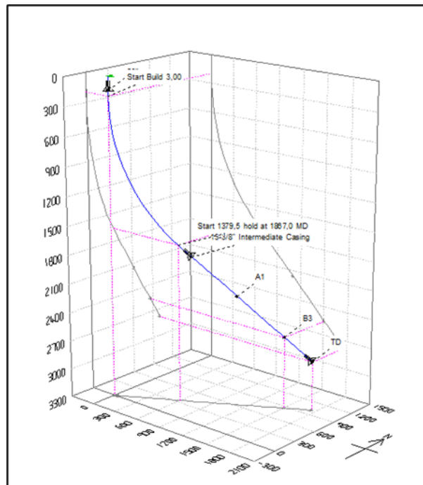
Gambar 10. Perencanaan Trajectory Sumur MST-01 3D View
