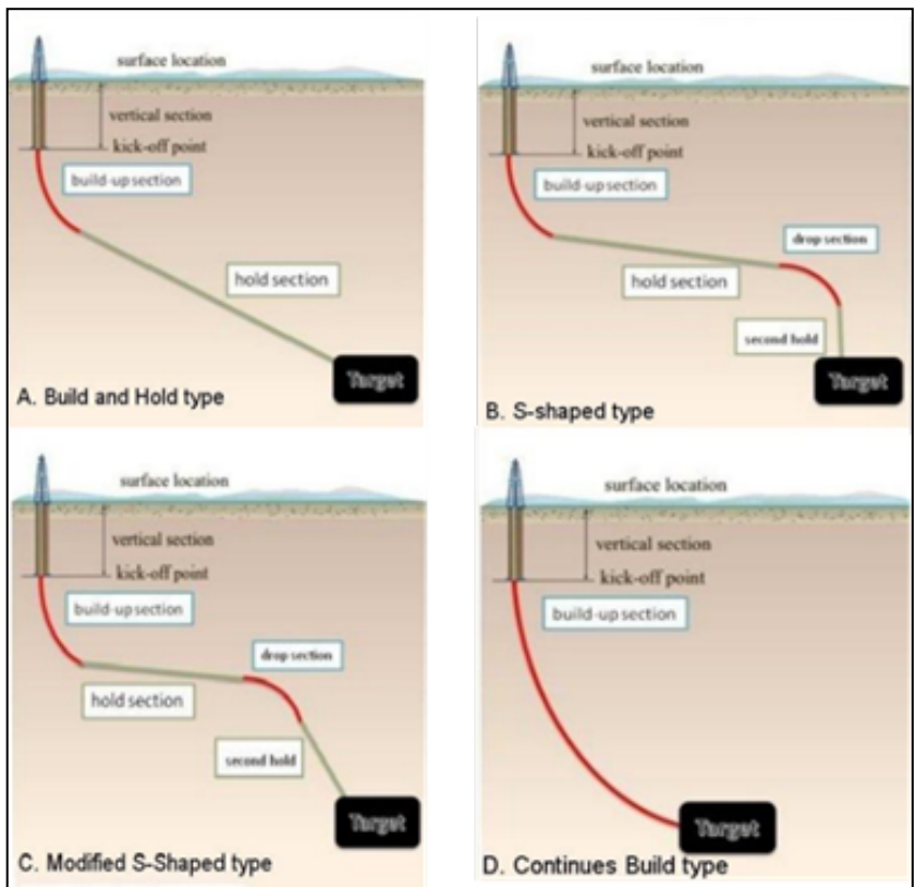
Gambar 1. Tipe Sumur Directional Drilling (Musa et al, 2017)
