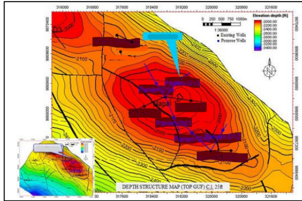
Gambar 2. Depth Structure Well MST-01, Sumber: Data Penelitian
