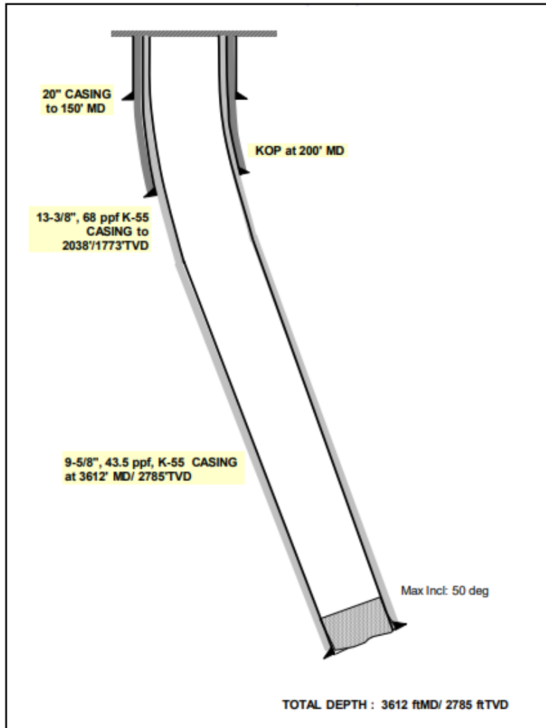
Gambar 4. Well Profile MST-01 Sumber: Data Penelitian
