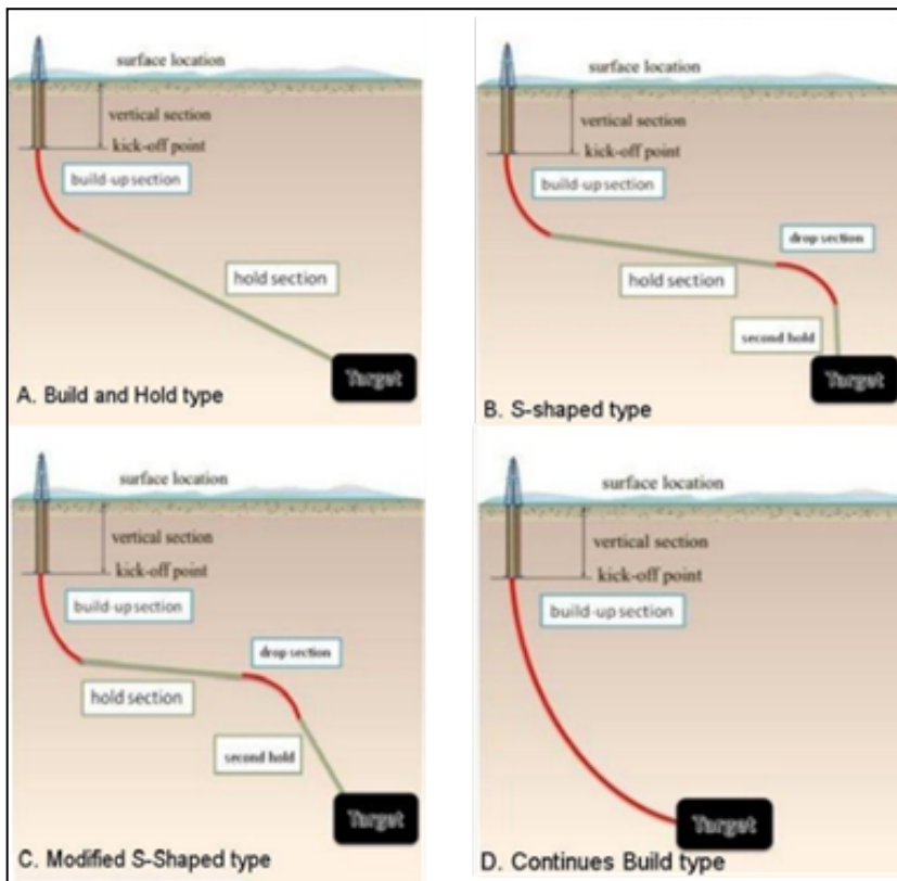
Gambar 1. Tipe Sumur Directional Drilling (Musa et al, 2017)
