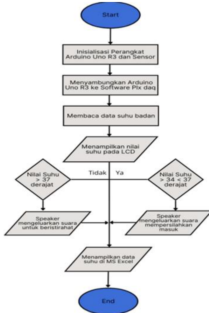
Gambar 2. Flowchart Sistem
