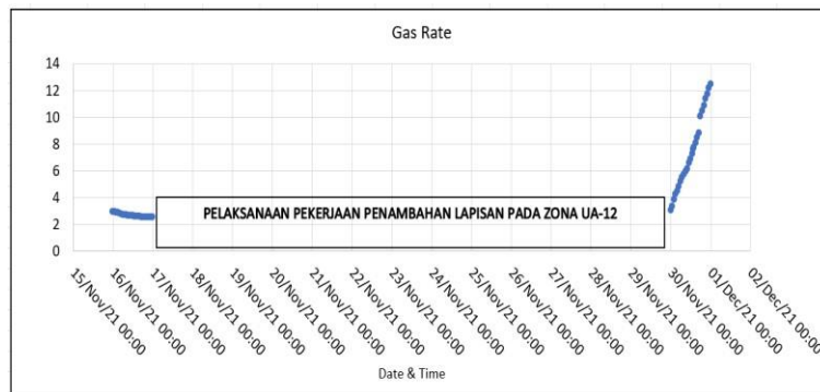
Gambar 1. Grafik Gas Rate Before and after Open SSD
