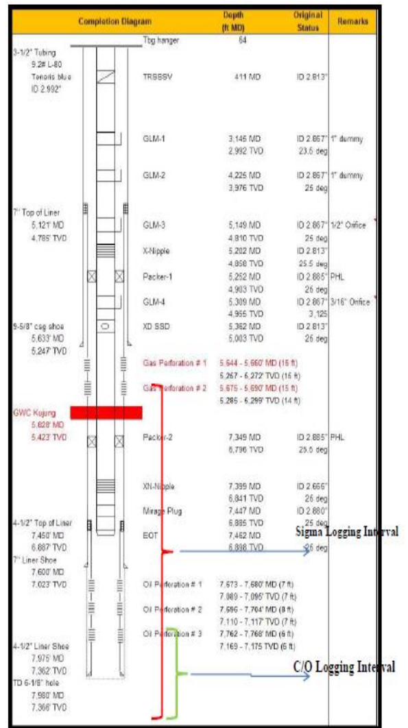
Gambar 3 Well Diagram
